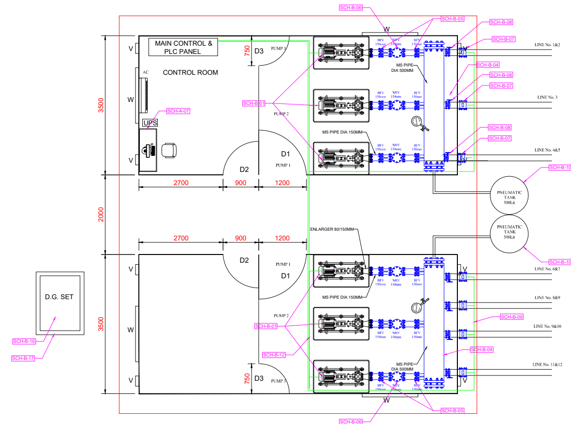
LAYOUT OF PUMPING ARRANGEMENT DELIVERY LINE
