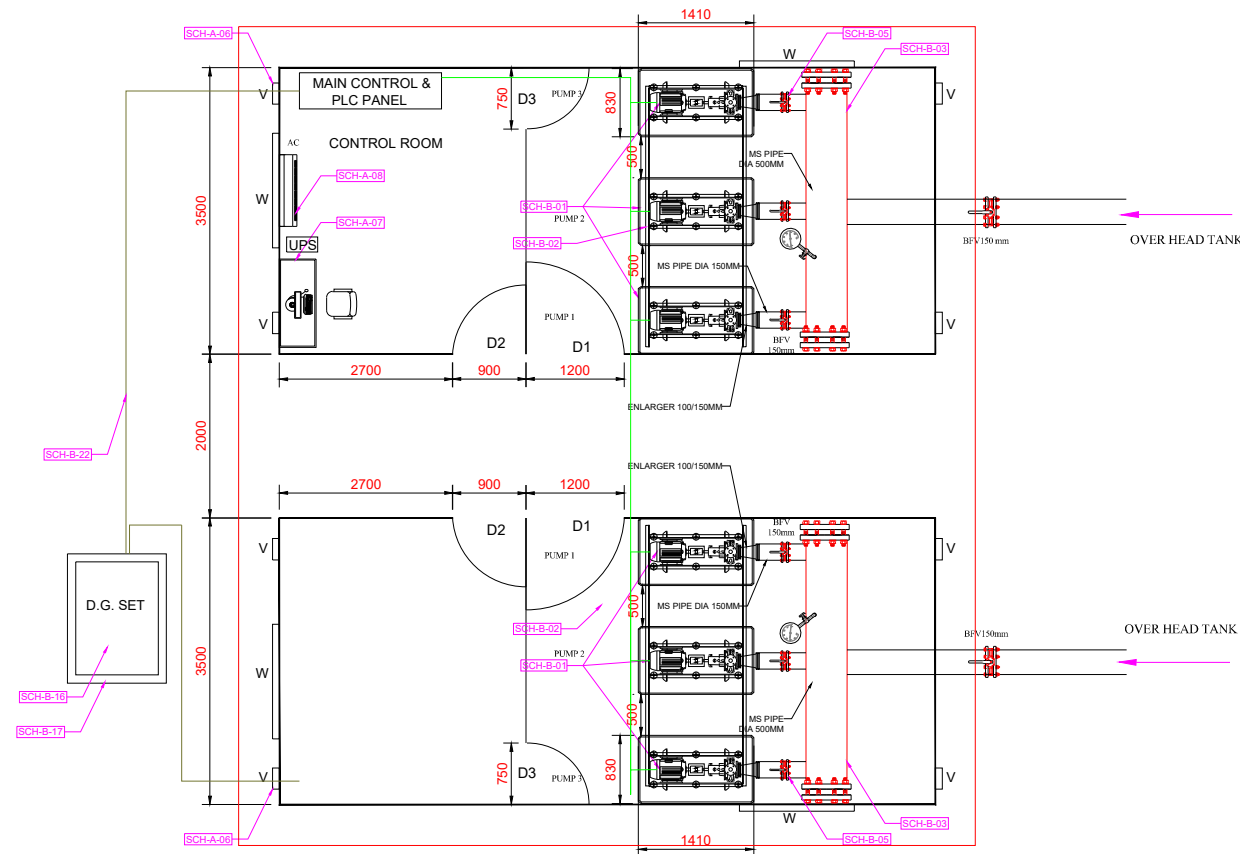
LAYOUT OF PUMPING ARRANGEMENT SUCTION LINE
