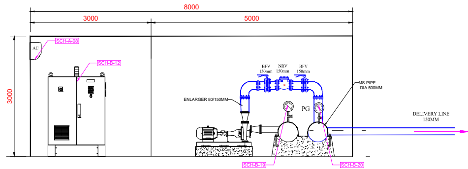
SIDE VIEW OF PUMPING ARRANGEMENT
