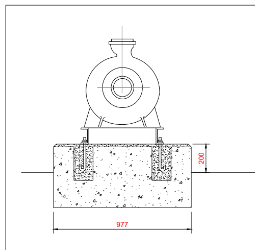
LAYOUT OF PUMPING ARRANGEMENT SUCTION LINE
